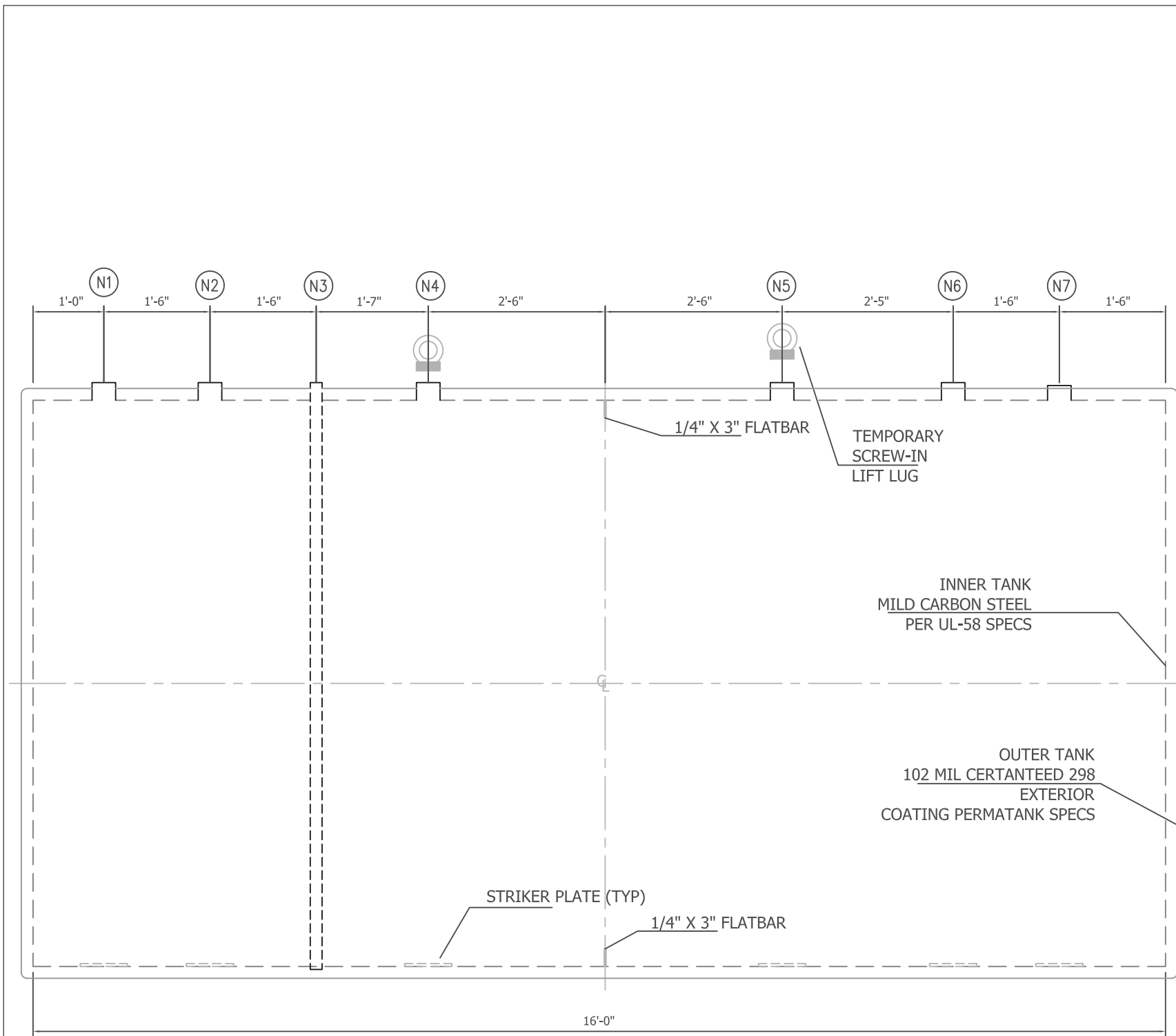
SIDE ELEVATION
