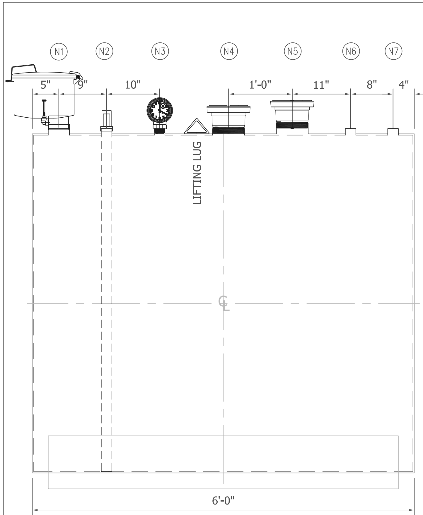
SIDE ELEVATION
